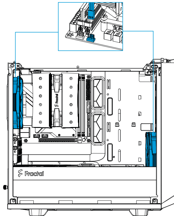
Chassis Fans
