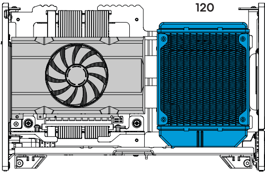
GPU max length 200 mm
